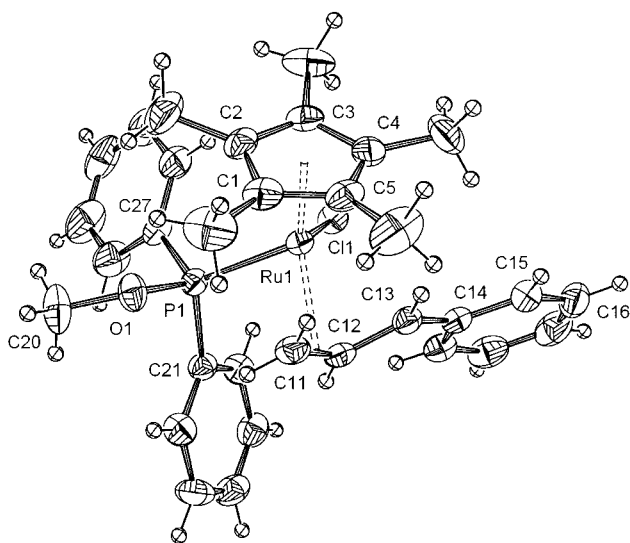
Figure 3. ORTEP drawing of 8e showing 50% probability thermal ellipsoids. The \text{PF}_6 anion is omitted for clarity. Selected bond lengths [Å] and angles [°]: Ru1–C11 2.182(5), Ru1–C12 2.210(4), Ru1–C13 2.452(4), C11–C12 1.398(6), C12–C13 1.396(6), C13–C14 1.457(6), Ru1–P1 2.360(1); C11–C12–C13 119.5(4), C12–C13–C14 125.7(4).
