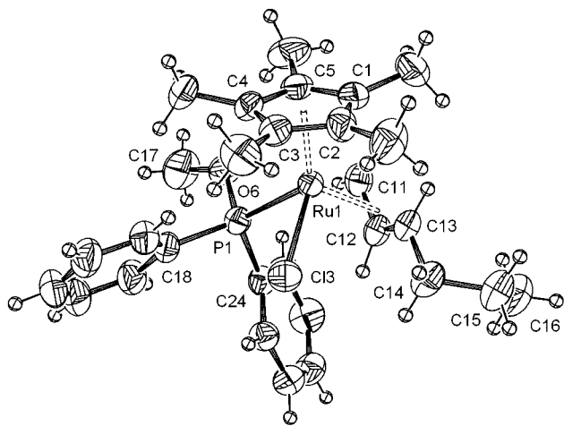
Figure 2. ORTEP drawing of 8d showing 50% probability thermal ellipsoids. The \text{PF}_6 anion is omitted for clarity. Selected bond lengths [Å] and angles [°]: Ru1–C11 2.191(4), Ru1–C12 2.198(4), Ru1–C13 2.339(4), Ru1–P1 2.368(1), C11–C12 1.406(6), C12–C13 1.395(6), C13–C14 1.497(6), Ru1–P1 2.368(1); C11–C12–C13 119.1(4), C12–C13–C14 123.7(4).
